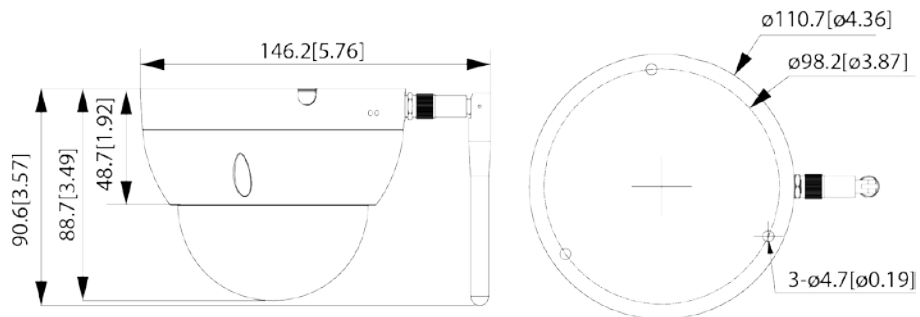
Figure 4-2 Dimensions (mm [inch])
